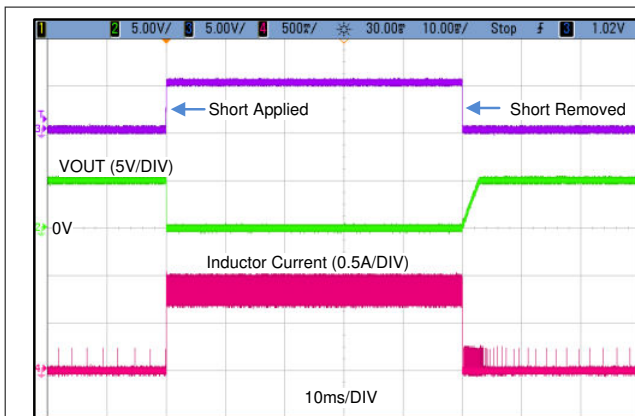
图 8-12. Short Circuit Waveform
