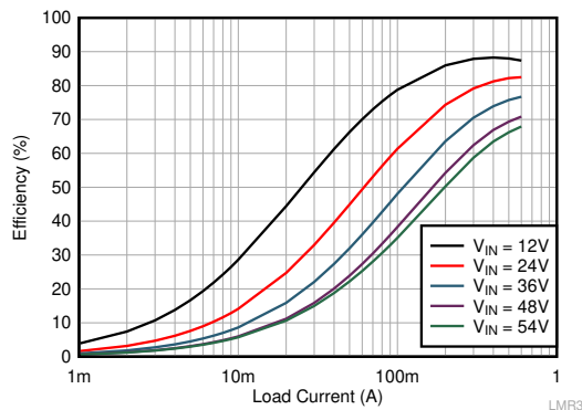
图 7-1. Efficiency 3.3-V Output, FPWM
