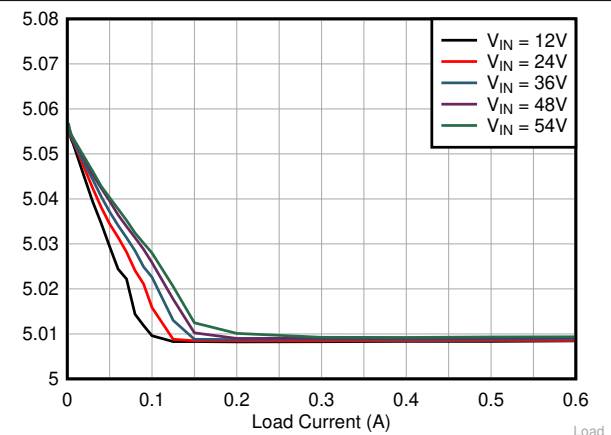
图 9-7. Line and Load Regulation
