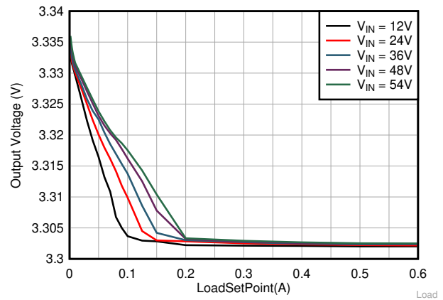
图 9-5. Line and Load Regulation
