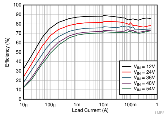
图 7-2. Efficiency 3.3-V Output, Auto Mode
