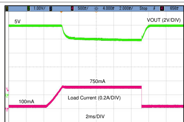
图 8-13. Overload Output Recovery (100 mA to 750 mA)
