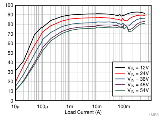
图 7-2. Efficiency 3.3-V Output, Auto Mode
