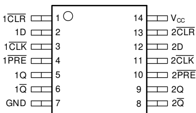
D and PW Package 14-Pin SOIC and TSSOP Top View
