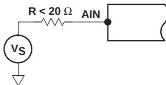
Figure 28. Damping Source Ringing Using a Small Resistor
