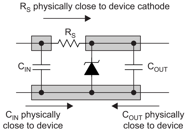
Figure 18. Layout Diagram
