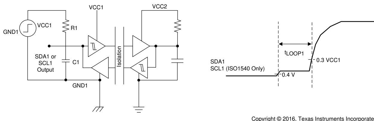
图 7-2. t_{\text{Loop1}} Setup and Timing Diagram
