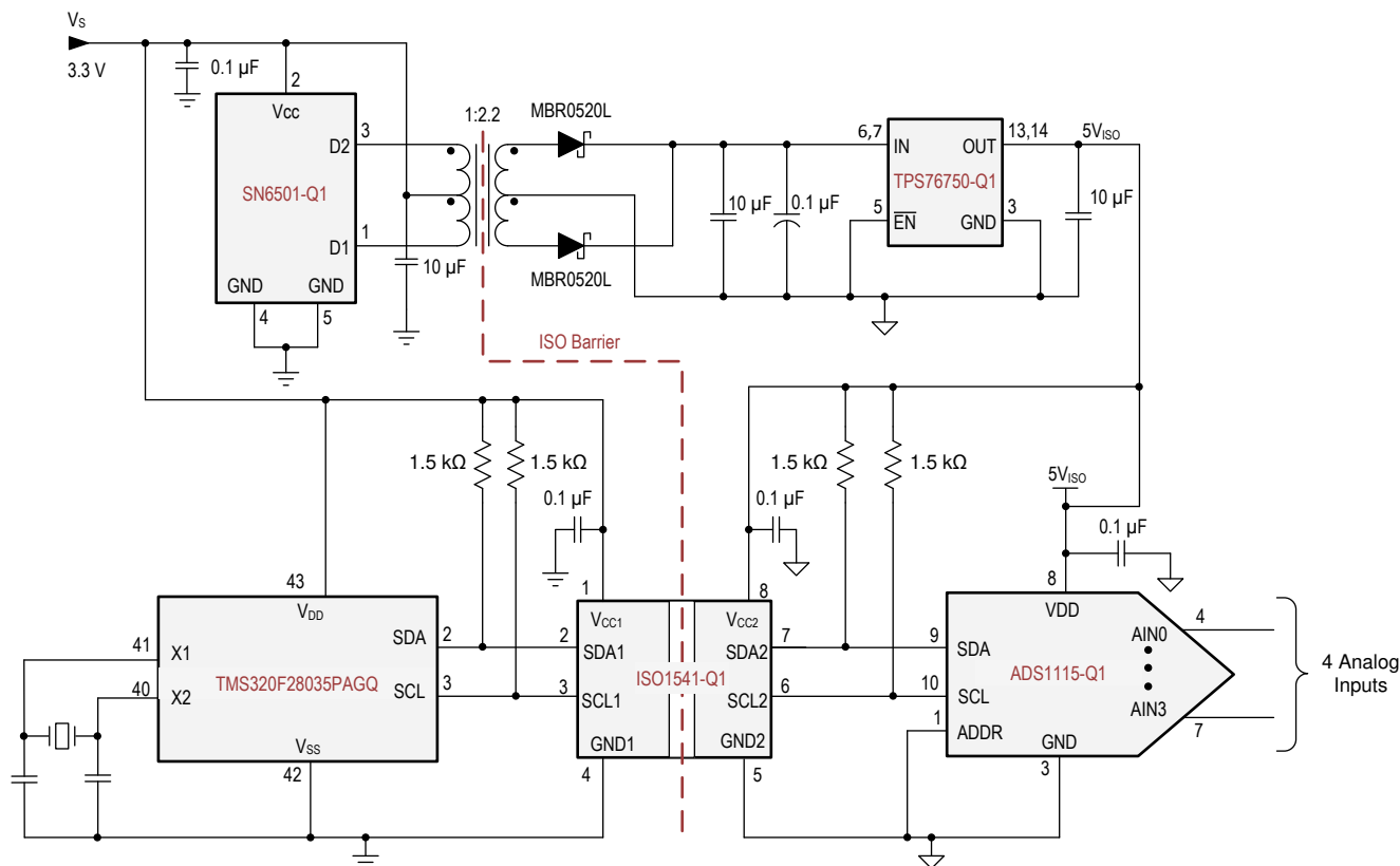
图 8-4. Isolated I²C Data Acquisition System
