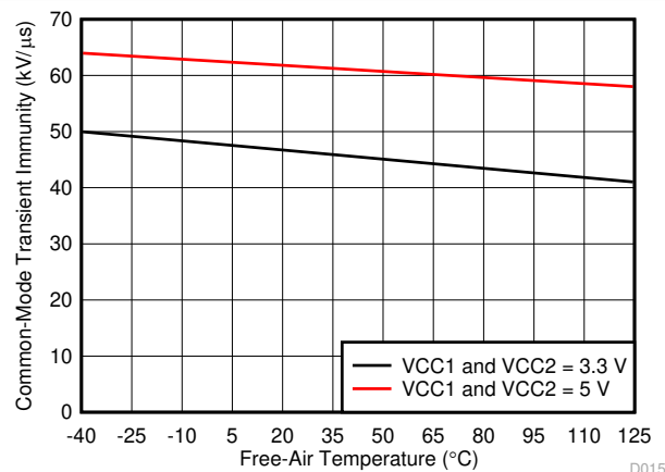
图 6-18. CMTI vs Free-Air Temperature
