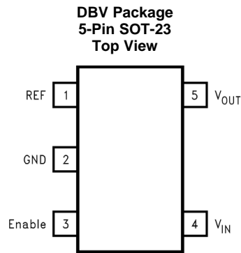
Pin Functions
