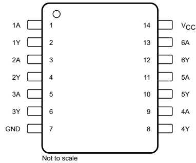
SOIC, SSOP, TVSOP, CDIP, PDIP, SO, TSSOP, or CFP Package 14-Pin D, DB, DGV, J, N, NS, PW, or W Top View
