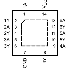
VQFN Package 14-Pin RGY Top View
