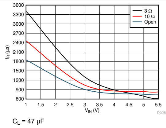
图 7-22. Rise Time vs Load Resistance (CT = 10000 pF)
