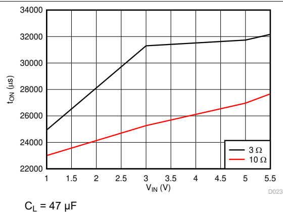
图 7-20. Turn-On vs Load Resistance (CT = 10000 pF)
