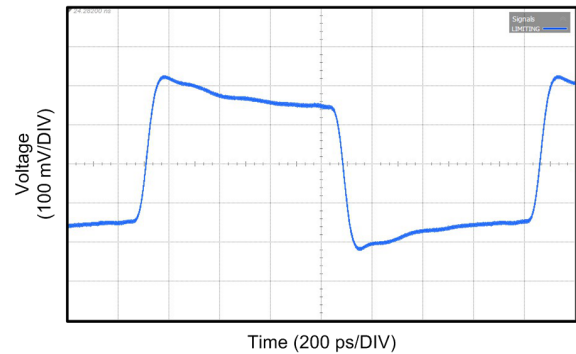
Figure 10. Example of TX De-emphasis for a DS125RT410 Operating at 10.3125 Gbps
