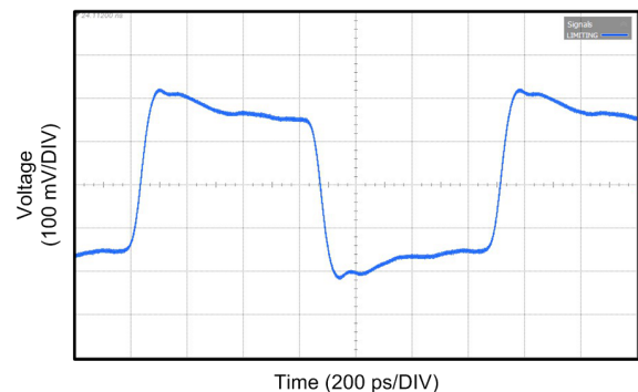
Figure 8. Example of TX De-emphasis for a DS125RT410 Operating at 12.5 Gbps
