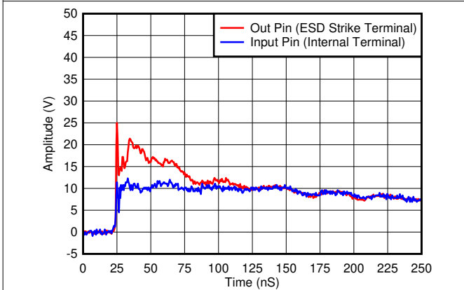
图 6-3. IEC Clamping Waveforms +8-kV Contact
