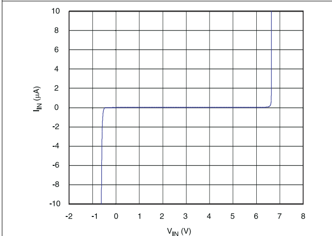
图 6-5. DC Characteristics ( I_{IN} vs V_{IN} ), T_A = 25^\circ\text{C}
