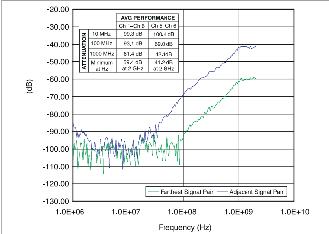
图 6-1. Channel-to-Channel Crosstalk
