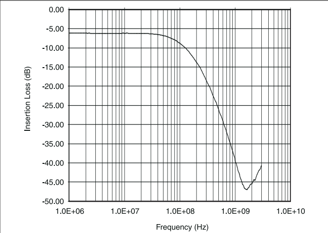
图 6-2. Frequency Response Data (0-V Bias)
