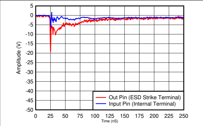
图 6-4. IEC Clamping Waveforms -8-kV Contact
