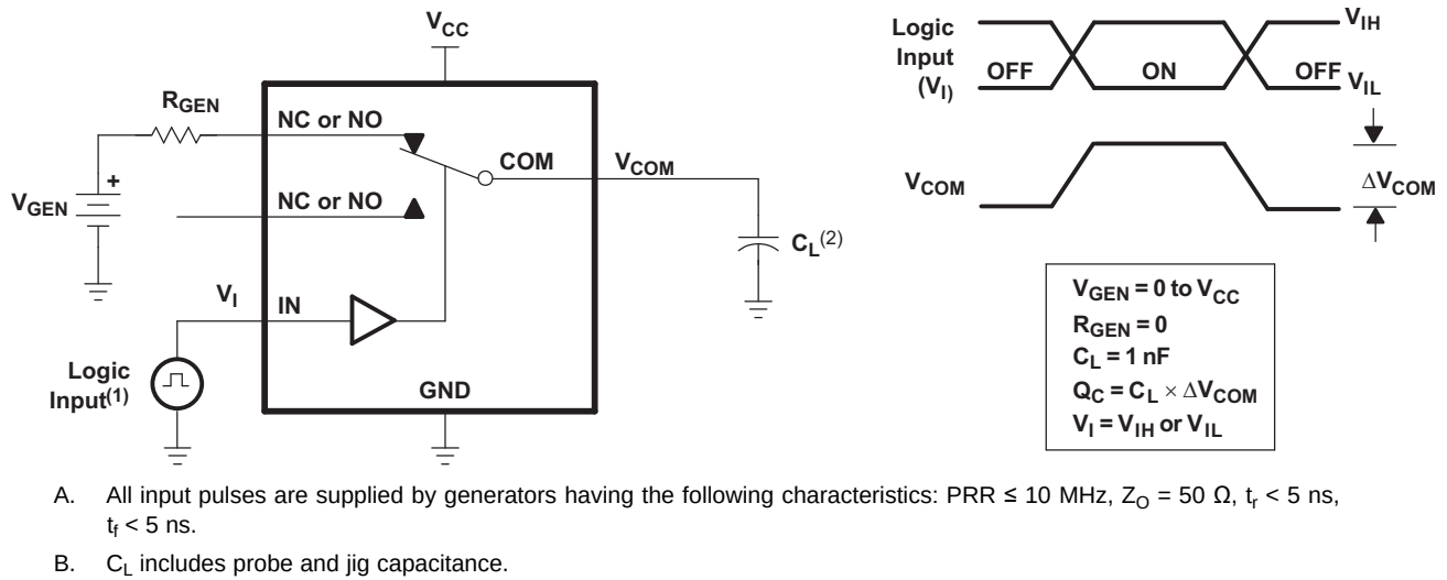
Figure 19. Charge Injection ( Q_C )
