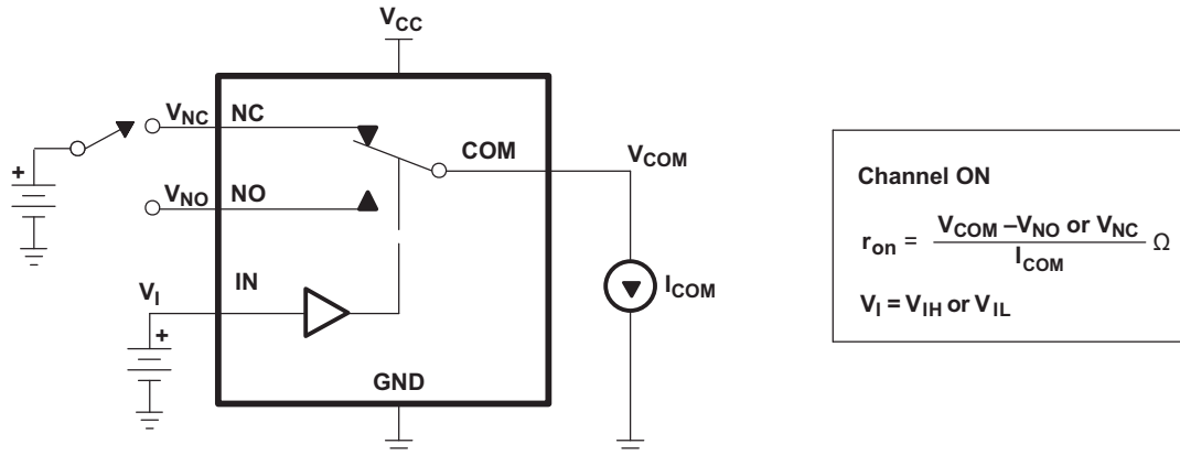
Figure 10. ON-State Resistance
