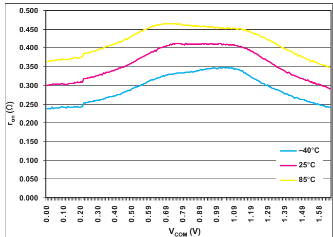
Figure 1. r_{on} vs V_{COM} ( V_{CC} = 1.65 V)
