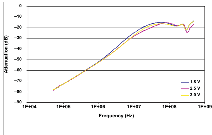
Figure 7. OFF Isolation
