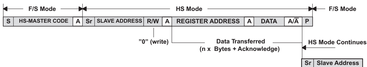
Figure 51. Data Transfer Format in H/S-Mode
