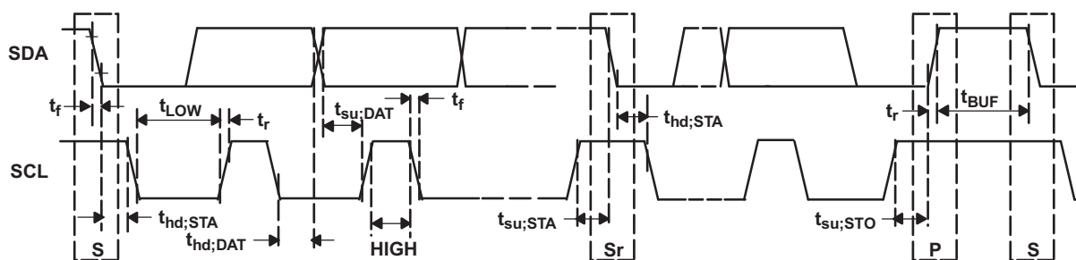
Figure 1. Serial Interface Timing Diagram for F/S-Mode
