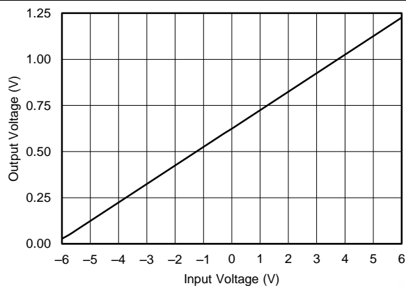
Figure 33. Output Code Error vs Input Voltage
