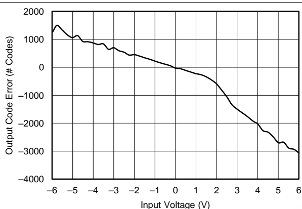
Figure 32. OPA317 Output Voltage Error vs Input Voltage
