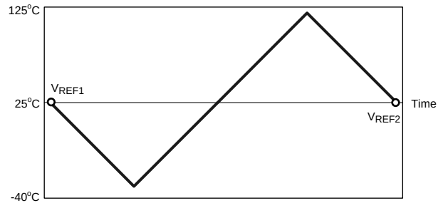
Figure 47. Temperature Profile
