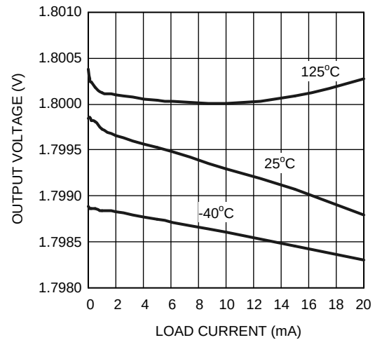
Figure 12. Load Regulation
