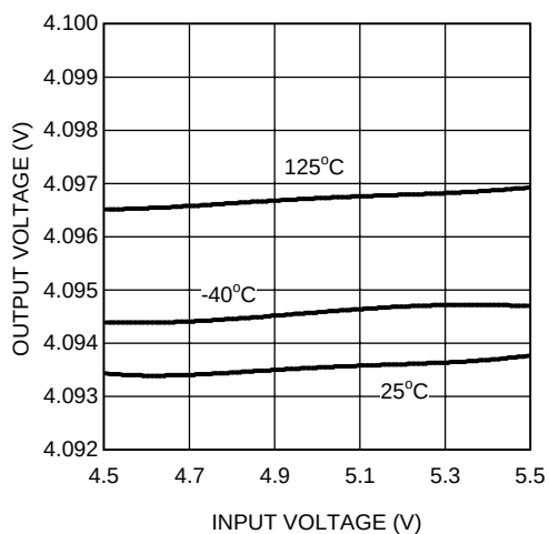
Figure 43. Line Regulation
