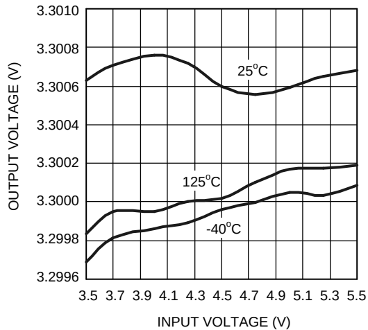
Figure 37. Line Regulation
