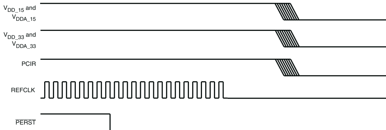
Figure 6-2. Power-Down Sequence
