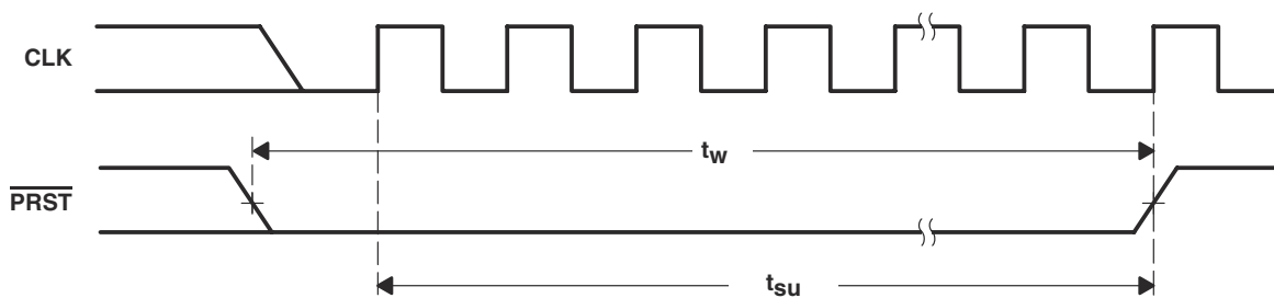
Figure 7-3. \overline{\text{PRST}} Timing Waveforms
