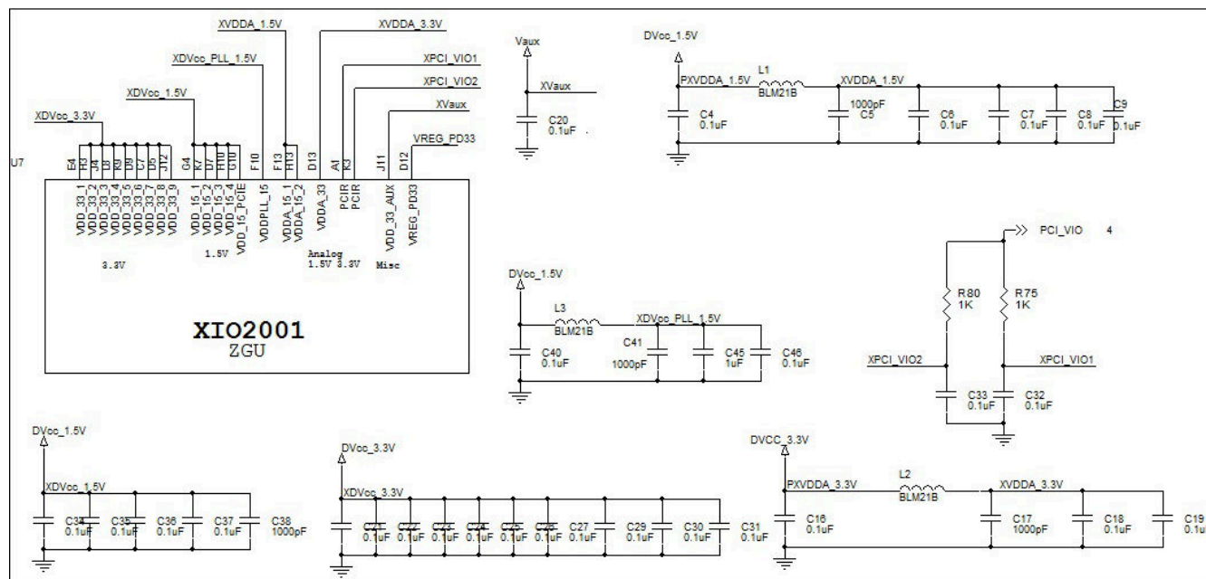
Figure 9-8. Power Filtering
