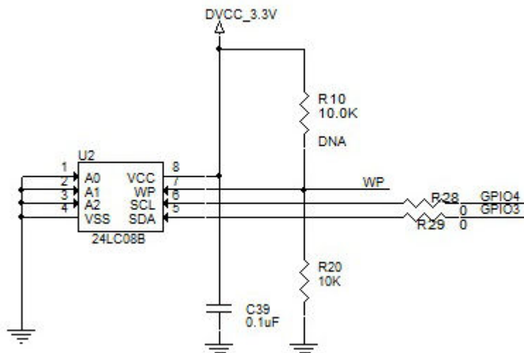
Figure 9-5. External EEPROM
