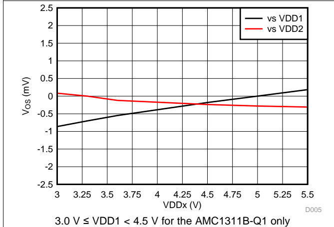
图 7. Input Offset Voltage vs Supply Voltage
