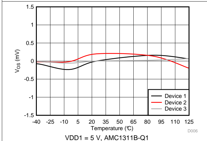
图 9. Input Offset Voltage vs Temperature
