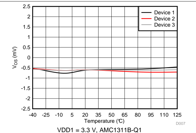
图 10. Input Offset Voltage vs Temperature
