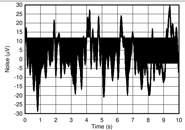
图 47. DAC Output Noise: 0.1 Hz to 10 Hz
