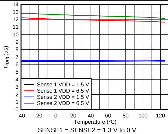
图 14. Propagation Delay from Sense Low to Output Low
