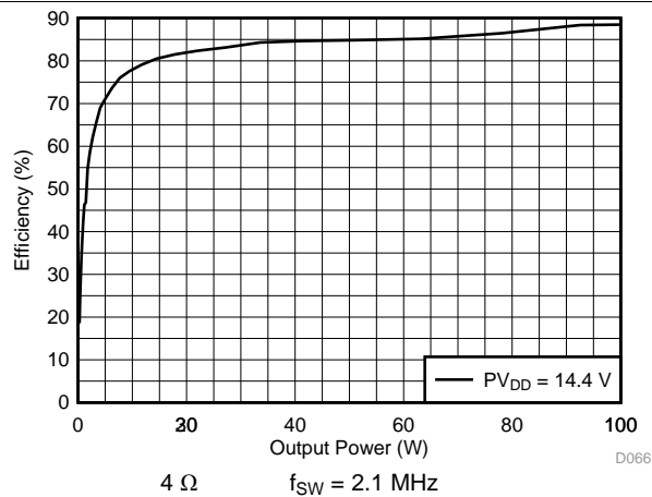
图 13. PVDD Power Efficiency vs Total Output Power
