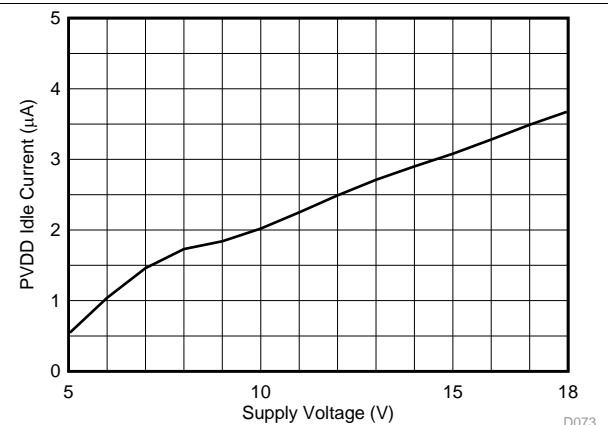
图 16. PVDD Idle Current vs Voltage
