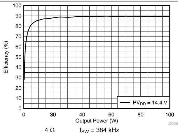
图 12. PVDD Power Efficiency vs Total Output Power
