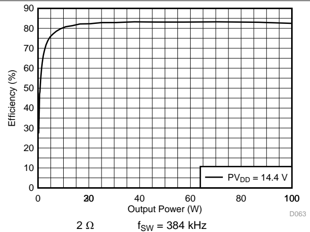
图 14. PVDD Power Efficiency vs Total Output Power
