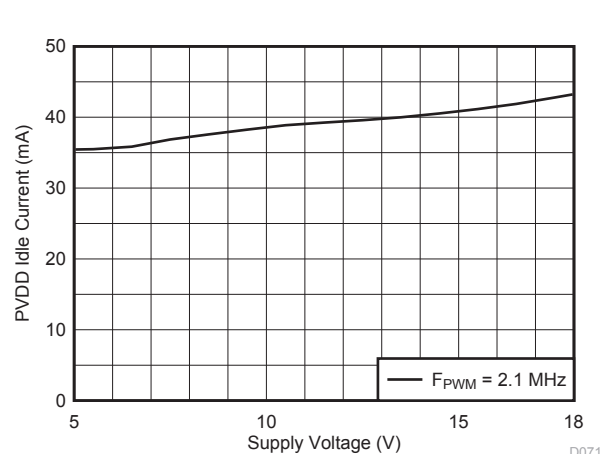
图 16. PVDD Idle Current vs Voltage
