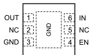
图 5-4. DRV Package, 6-Pin WSON, Top View
