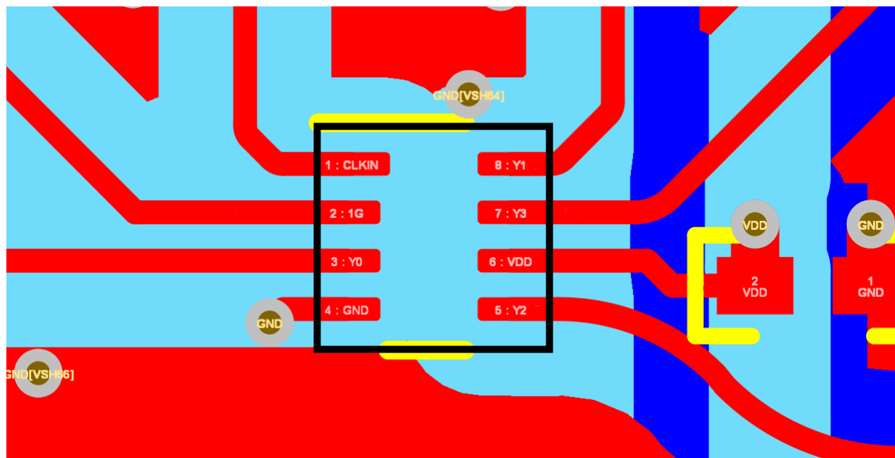
图 11-2. Layout illustration for 8-pin WSON device
