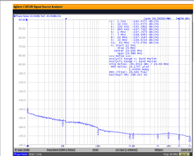
图 9-3. LMK1C110x 3.3-V Output Phase Noise 26.7-fs (12 kHz to 20 MHz)
