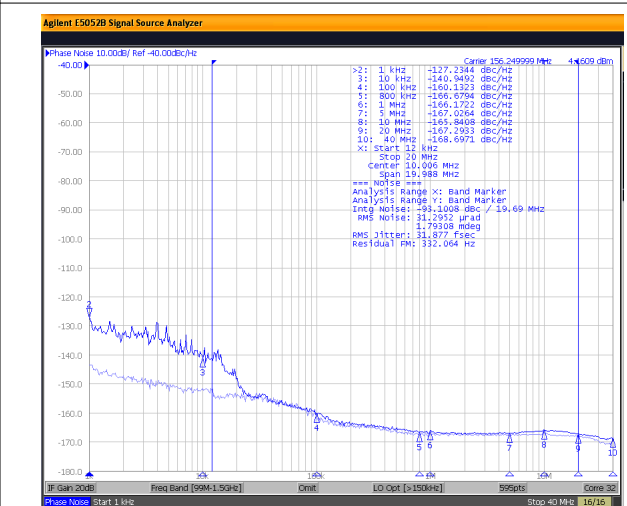
图 9-5. LMK1C110x 1.8-V Output Phase Noise 32-fs (12 kHz to 20 MHz)
