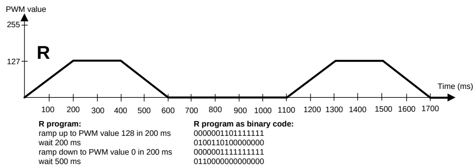
Figure 30. Sequence Diagram
