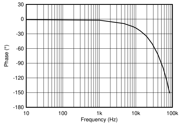
图 7-4. Phase vs. Frequency, All Gains
