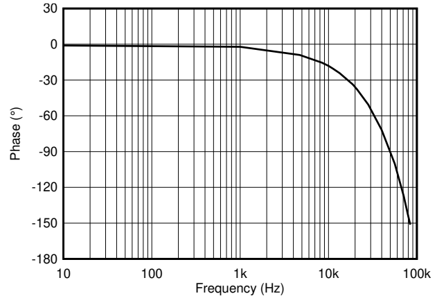
图 9-5. Normalized Phase, All Variants
