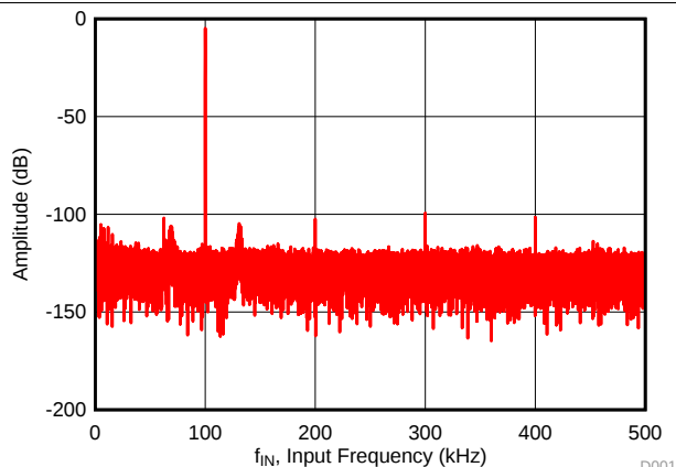
Figure 4. Typical FFT
