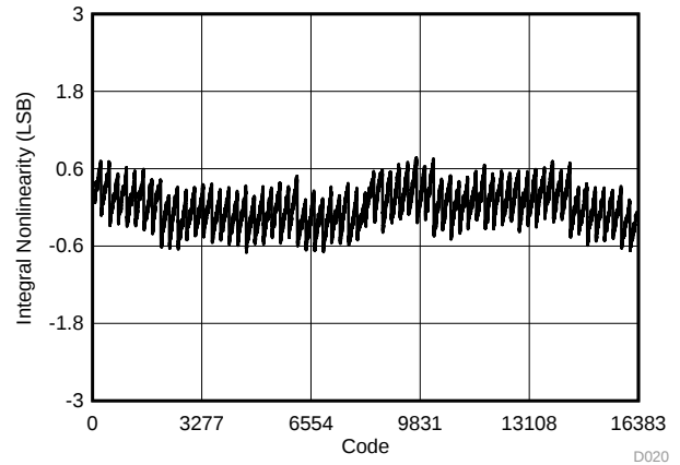
Figure 16. Typical INL
