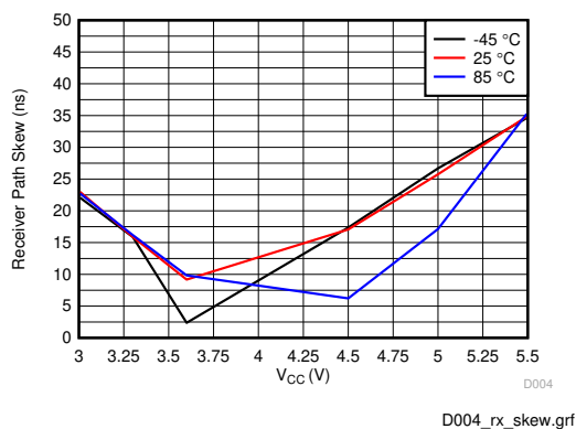
图 6-7. Receiver Path Skew ( |t_{pHL} - t_{pLH}| ) (RGT Package)
