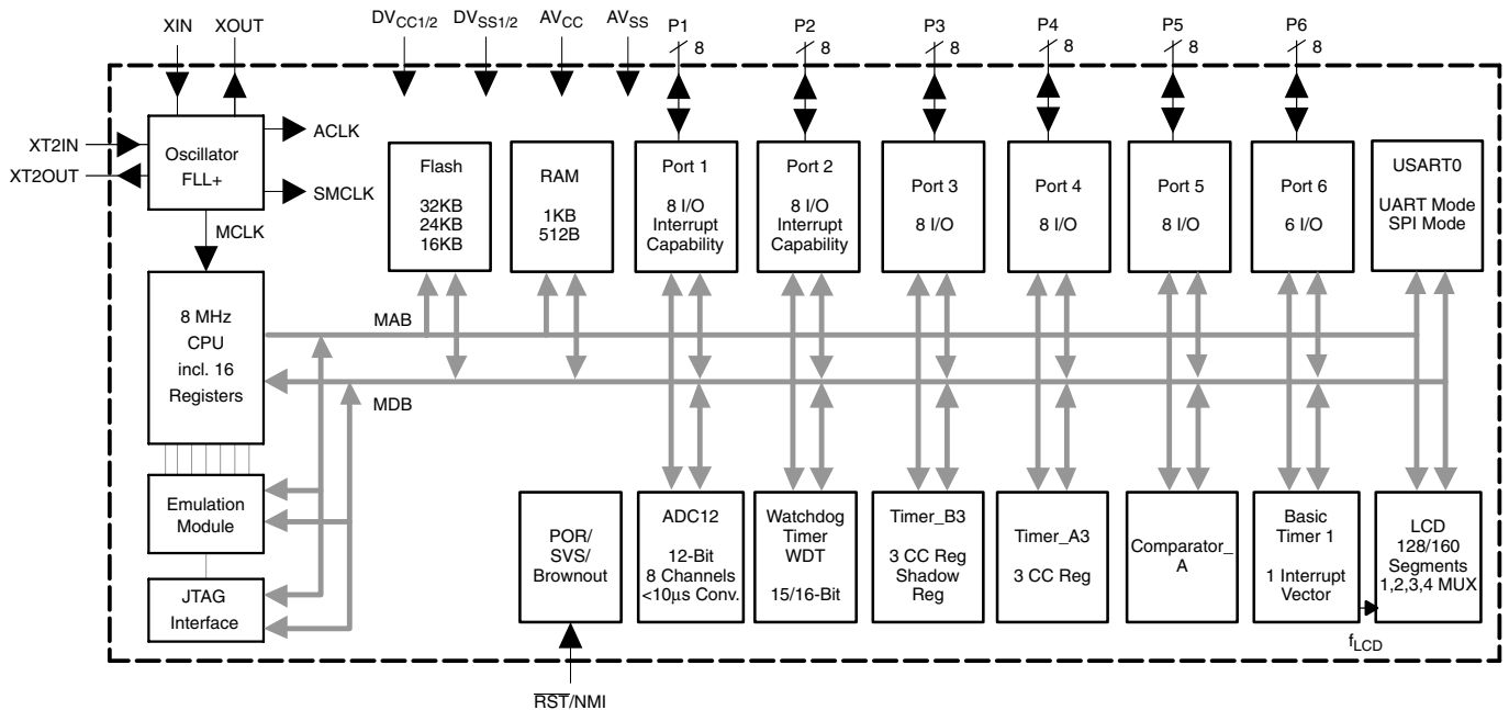
MSP430x43x functional block diagram
