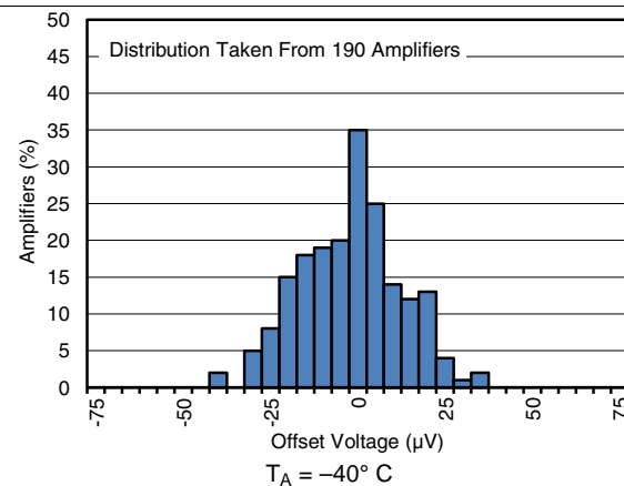
Figure 6. Offset Voltage Production Distribution at -40^\circ\text{C}
