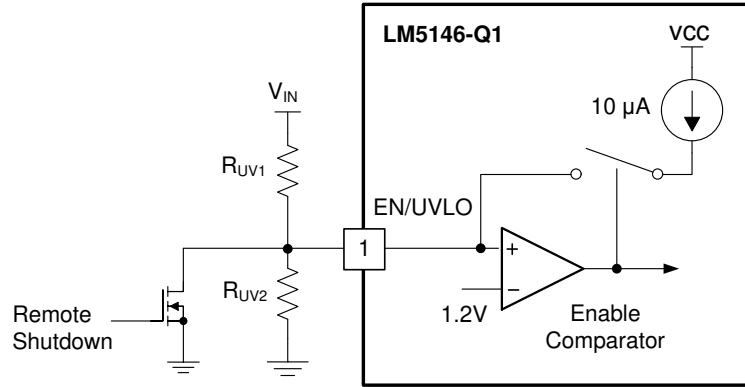
图 8-3. Programmable Input Voltage UVLO Turn-on and Turn-off
