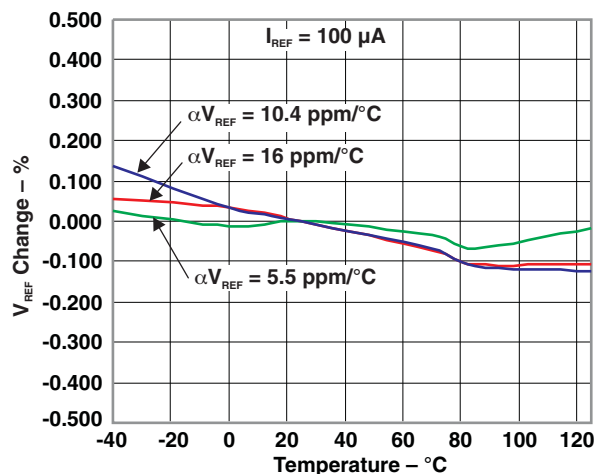
TEMPERATURE DRIFT FOR DIFFERENT AVERAGE TEMPERATURE COEFFICIENTS
