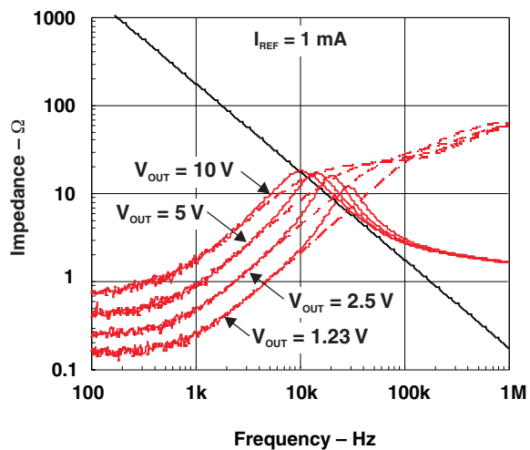
OUTPUT IMPEDANCE vs FREQUENCY
