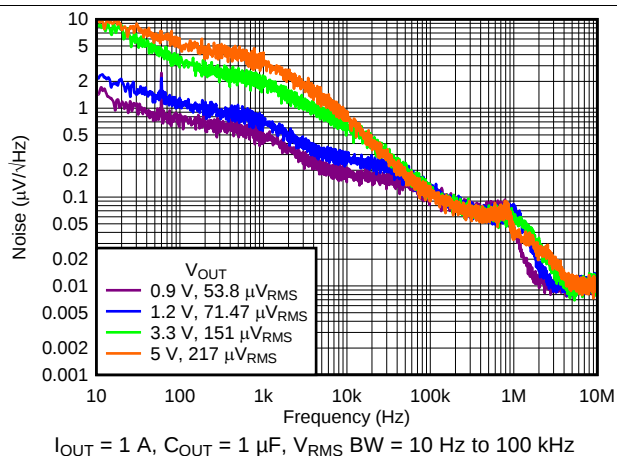
图 6. Output Noise vs Frequency and V_{OUT}
