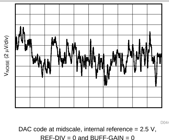
图 46. DAC Output Noise 0.1 Hz to 10 Hz
