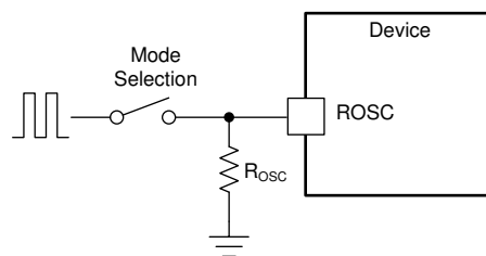
图 31. Works With Resistor Mode and Synchronization Mode
