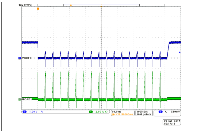
图 46. BUCK1 Hiccup and Recovery
