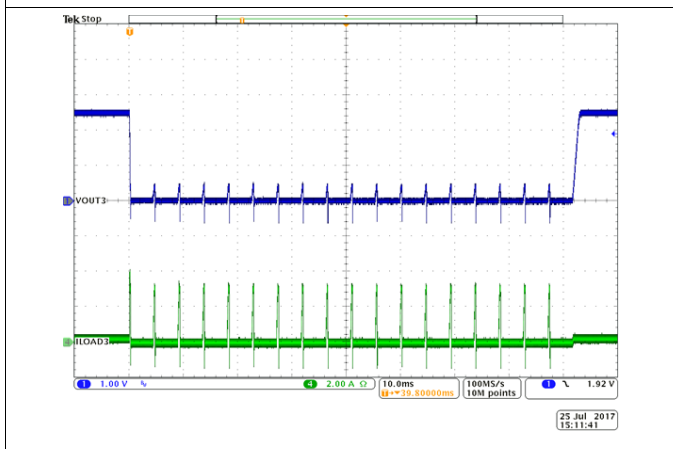
图 48. BUCK3 Hiccup and Recovery
