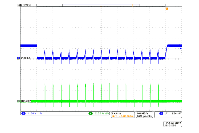
图 47. BUCK2 Hiccup and Recovery
