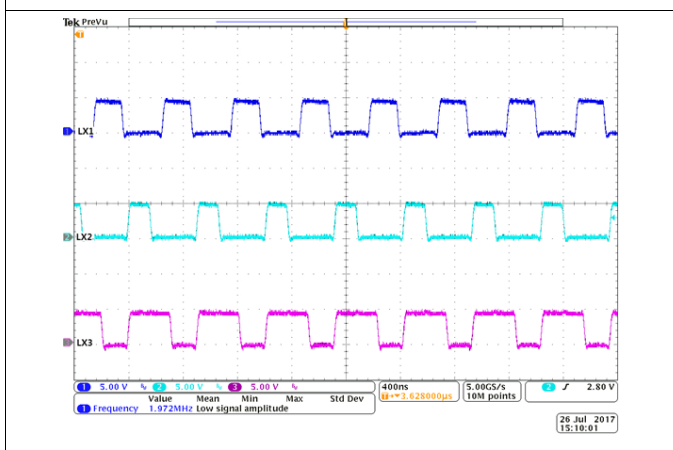
图 50. 180° Out-of-Phase
