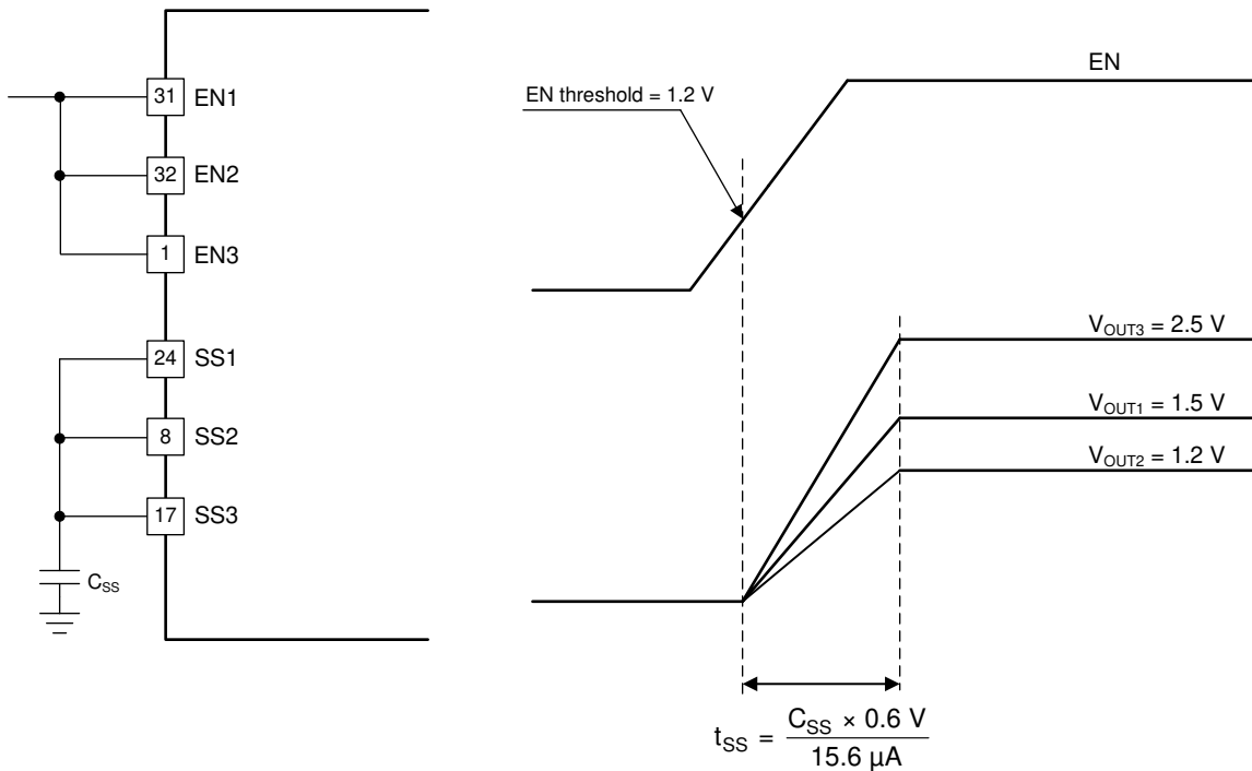
图 25. Ratiometric Power-Up Using SSx Pins
