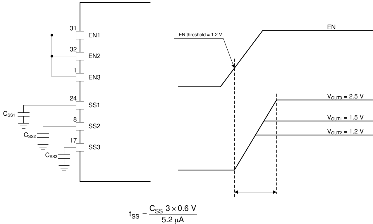
图 26. Simultaneous Startup Sequence Using SSx Pins
