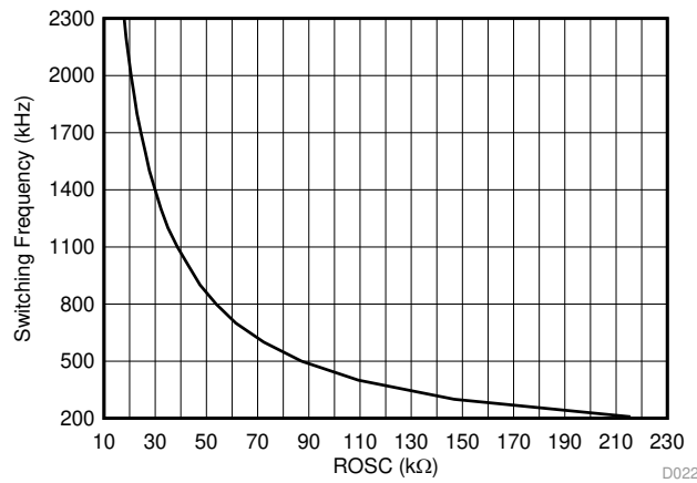
图 30. ROSC vs Switching Frequency
