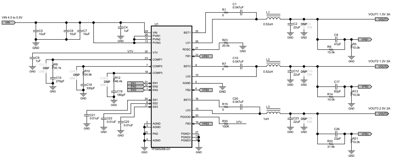
图 32. Typical Application Schematic
