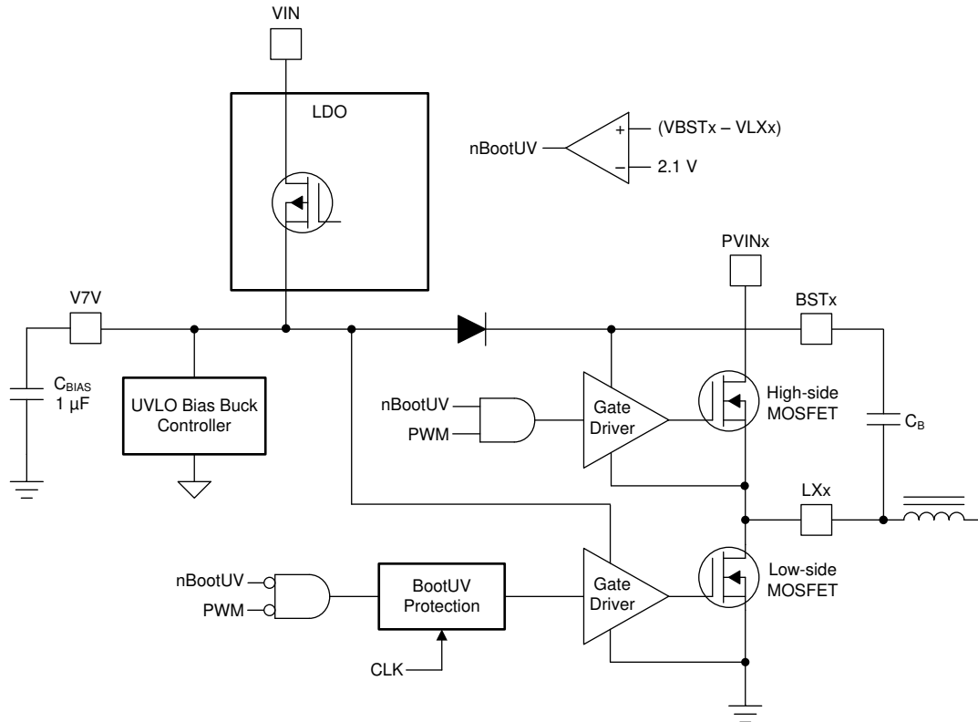
图 28. V7V Linear Dropout Regulator and Bootstrap Voltage Diagram
