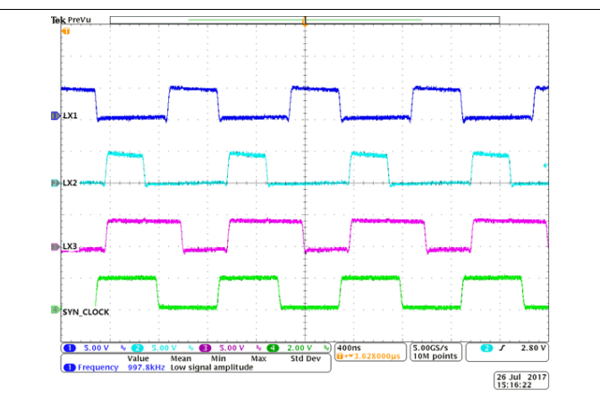
图 51. Synchronization With External Clock
