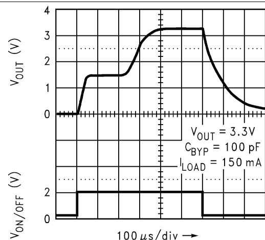
Figure 36. Turnon Time
