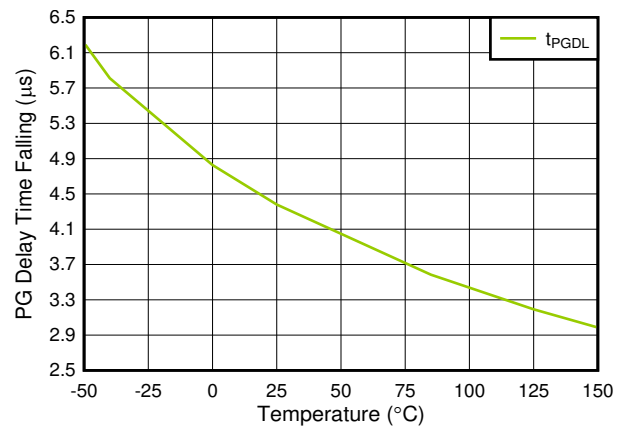
Figure 6-20. t_{PGDL} vs Temperature
