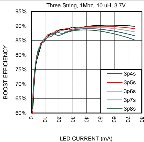
图 44. Boost Efficiency vs Series LEDs
