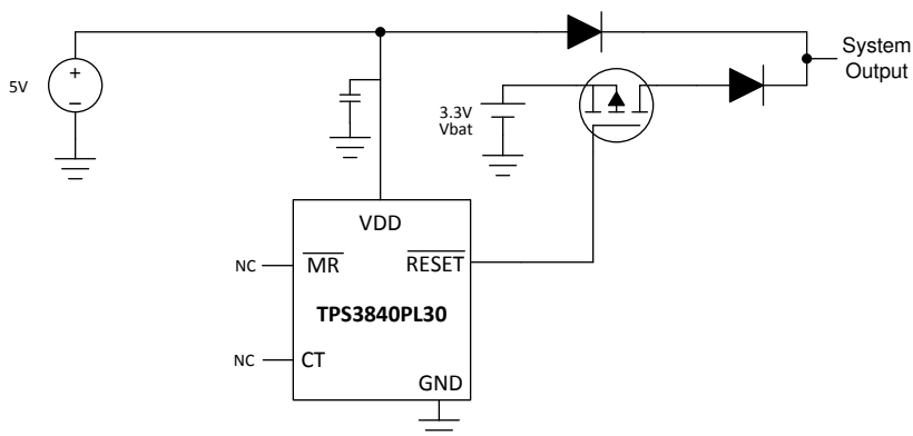
图 52. Voltage Monitor with Back-up Battery Switchover Solution
