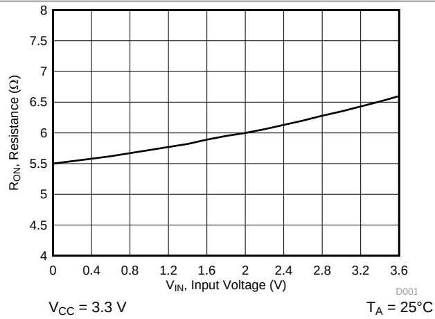
图 1. ON-Resistance vs Input Voltage
