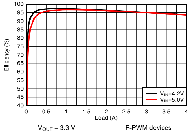
图 9-21. PWM Efficiency
