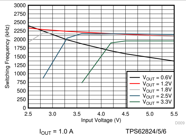
图 9-24. Switching Frequency
