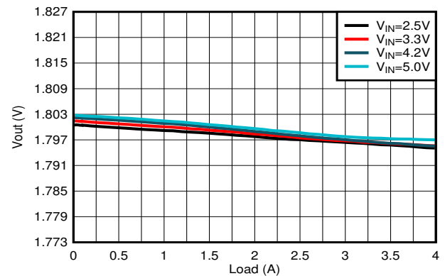
图 9-12. Load Regulation
