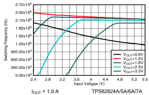
图 9-26. Switching Frequency
