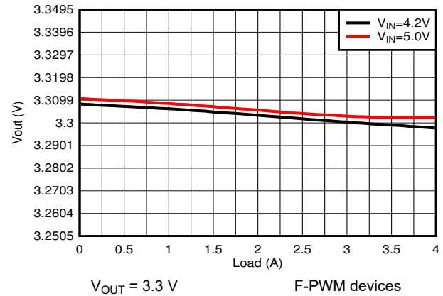
图 9-22. Load Regulation
