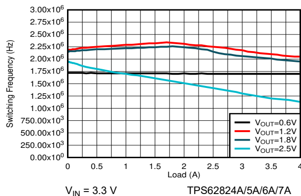
图 9-25. Switching Frequency
