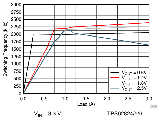
图 9-23. Switching Frequency
