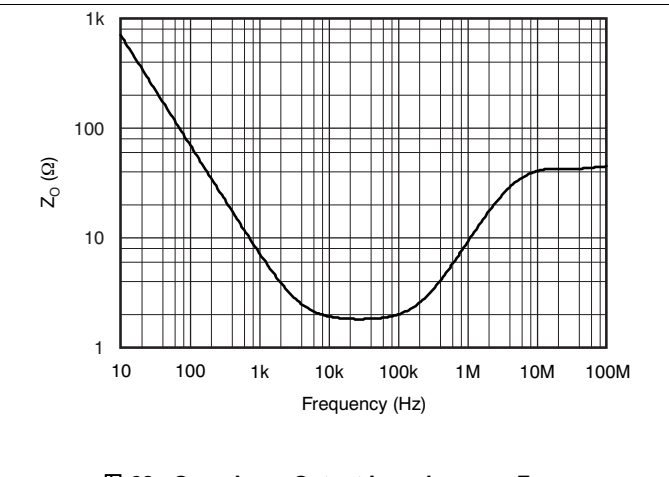
图 28. Open-Loop Output Impedance vs Frequency
