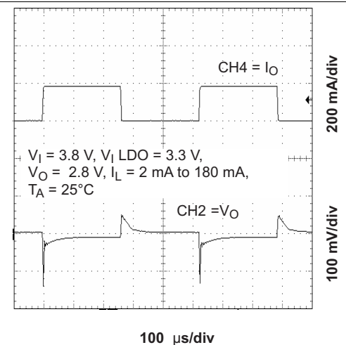
Figure 17. Line Transient Response (LDO1)
