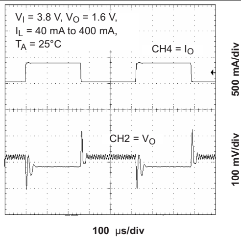
Figure 15. Line Transient Response (CORE)
