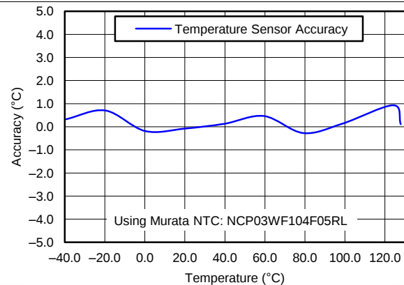
Figure 3. Temperature Accuracy
