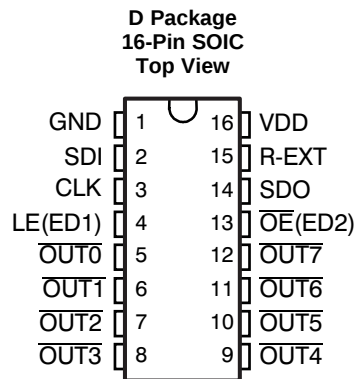
Pin Functions
