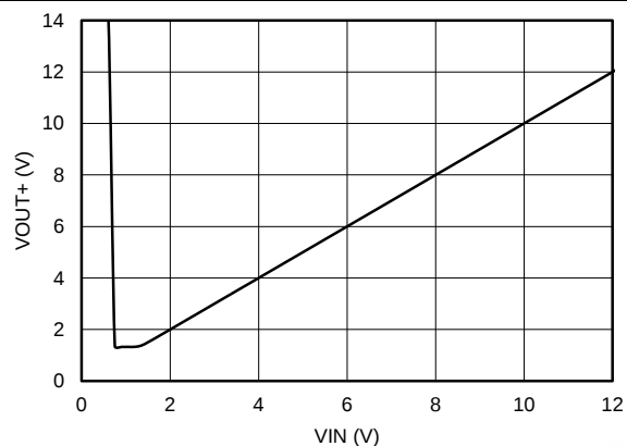
Figure 15. Positive Output Voltage vs Input Voltage
