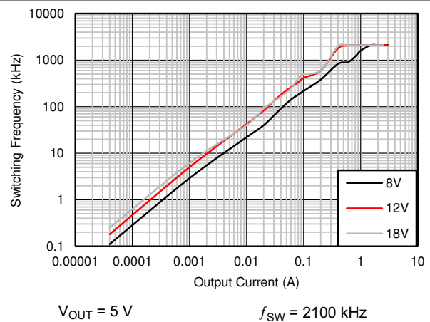
图 8-14. Switching Frequency versus Output Current
