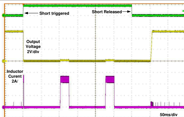
图 7-6. Short-Circuit Transient and Recovery
