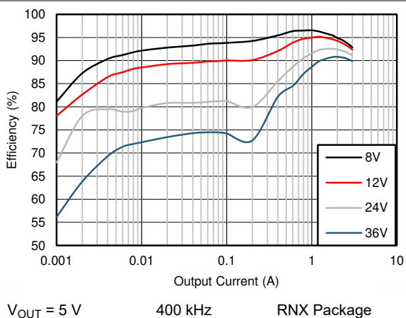
图 8-5. Efficiency
