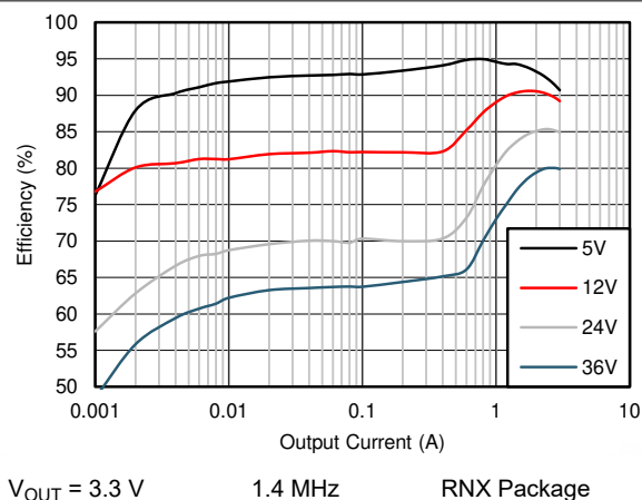
图 8-8. Efficiency
