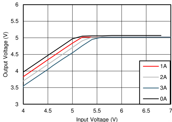
图 7-9. Overall Dropout Characteristic V_{OUT} = 5\text{ V}
