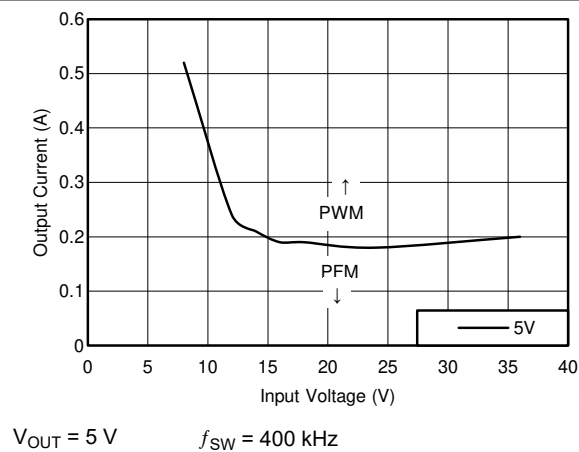
图 8-13. Mode Change Thresholds
