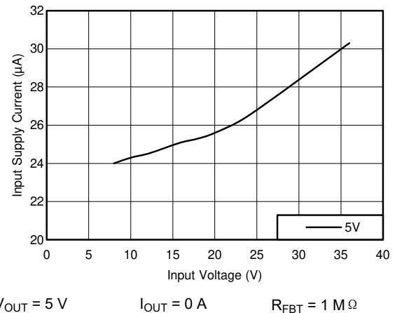
图 8-12. Input Supply Current
