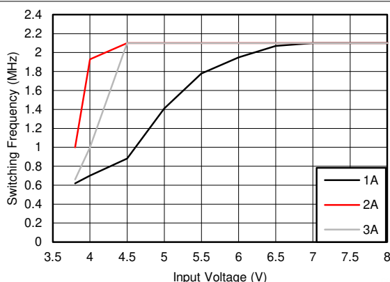
图 7-11. Typical Switching Frequency in Dropout Mode V_{OUT} = 3.3\text{ V} , f_{SW} = 2.1\text{ MHz}
