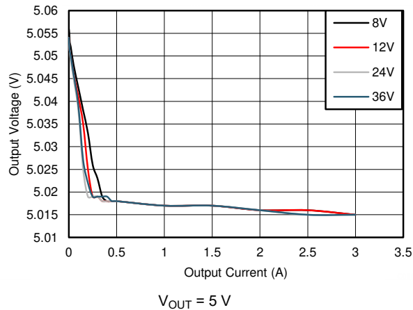
图 8-11. Line and Load Regulation
