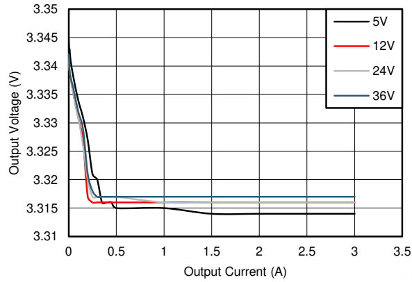
图 8-17. Line and Load Regulation
