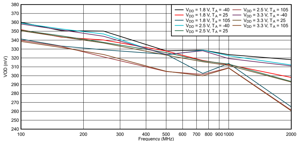
Figure 6-2. LMK1D1208 VOD vs. Frequency
