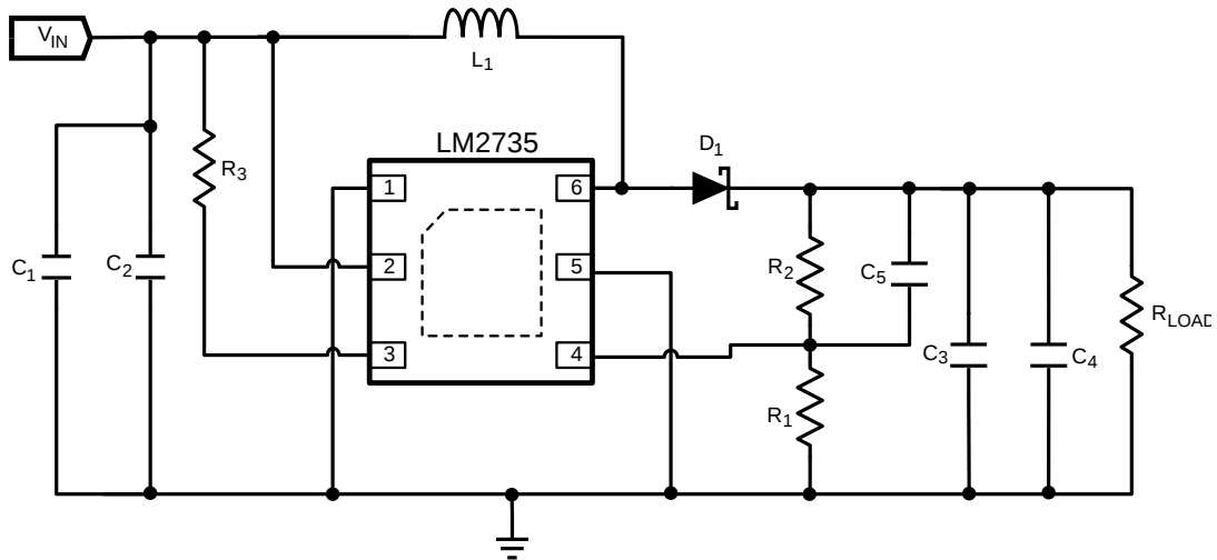
Figure 25. LM2735Y (520 kHz): V_{IN} = 3.3\text{ V} , V_{OUT} = 12\text{ V} at 350 mA
