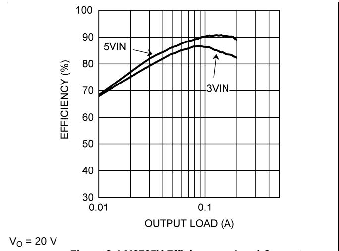
Figure 8. LM2735Y Efficiency vs Load Current
