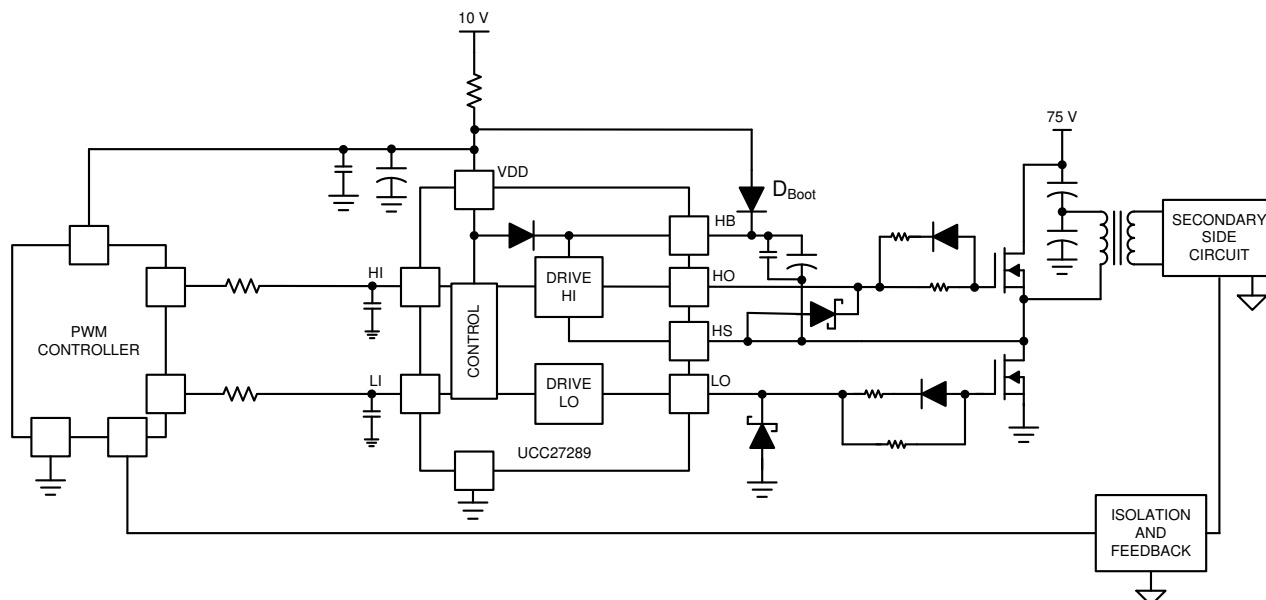
Figure 8-1. Typical Application
