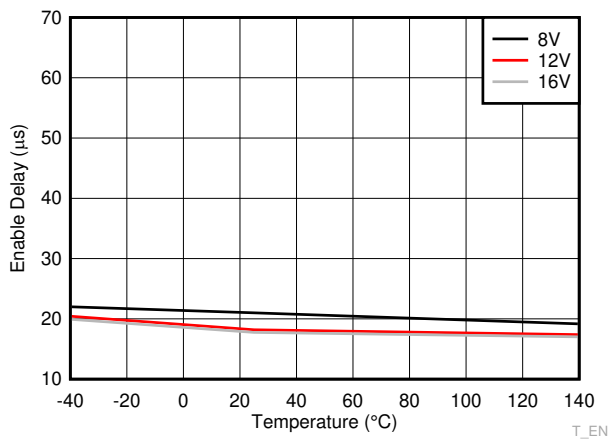
Figure 6-28. Enable Delay
