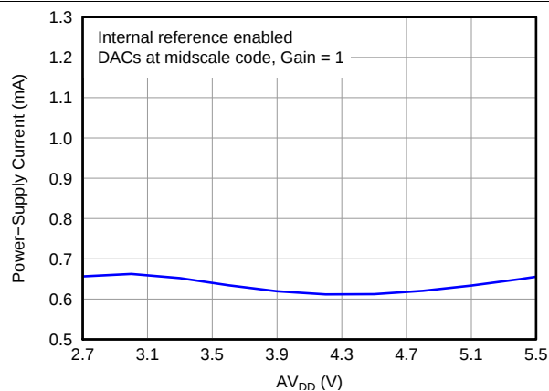
Figure 27. Power-Supply Current vs Power-Supply Voltage
