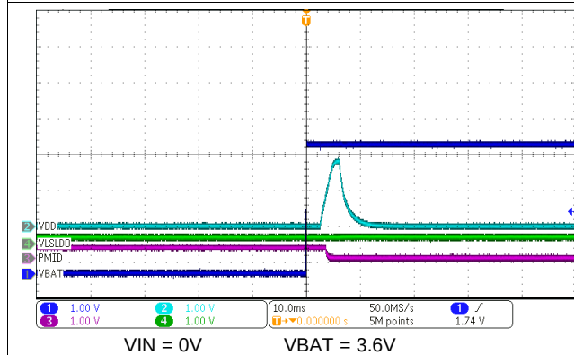
图 84. Wake In To Ship Mode on Battery Insertion with No IN Supply
