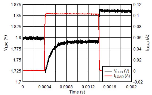
图 97. LDO Load Transient - VLDO = 1.8V
