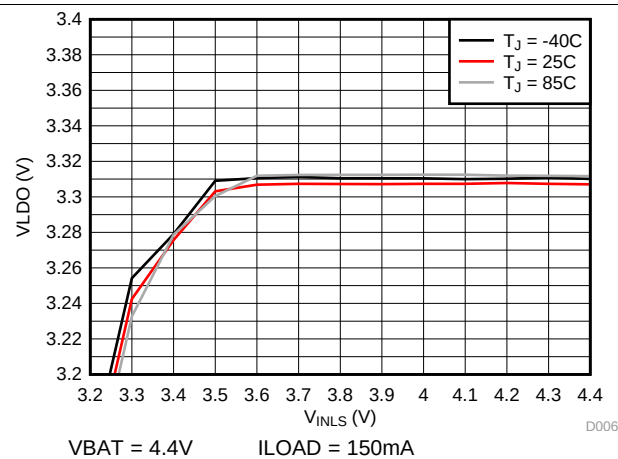
图 11. LDO Line Regulation ( V_{LDO} = 3.3V )
