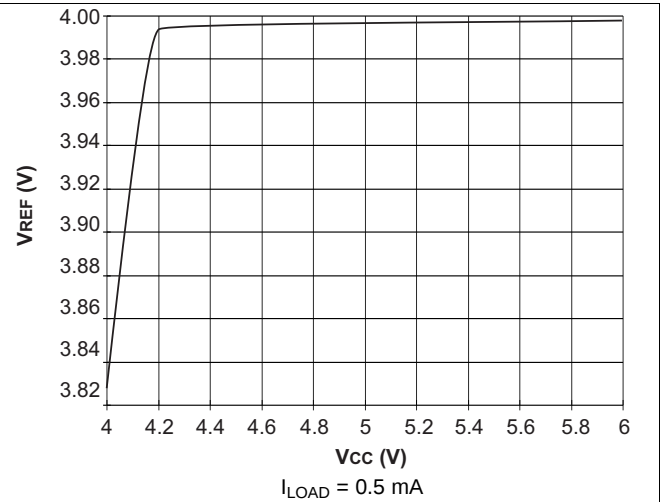
Figure 2. UCC2813-[3,5]-Q1: V_{REF} vs V_{CC}
