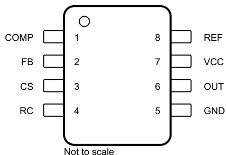
N and D Packages 8-Pin PDIP and SOIC Top View
