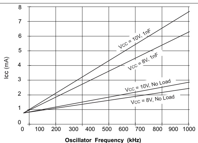
Figure 8. UCC2813-5-Q1: I CC vs Oscillator Frequency
